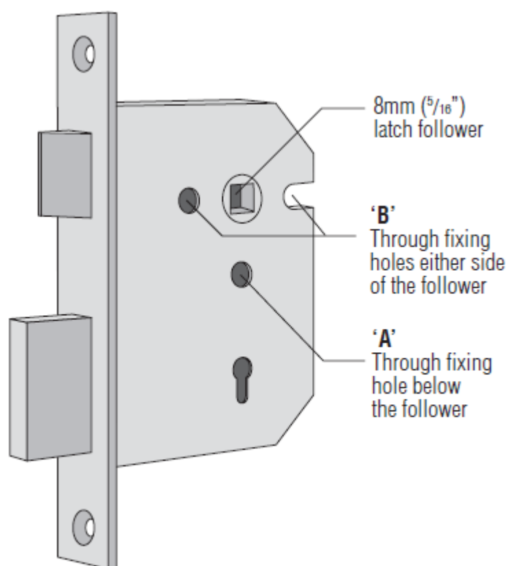
FIGURE 1 - Lock case
