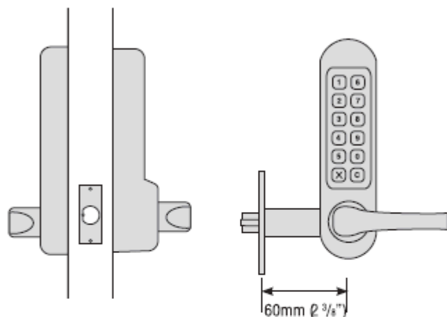
CL510/CL515 with tubular latchbolt
