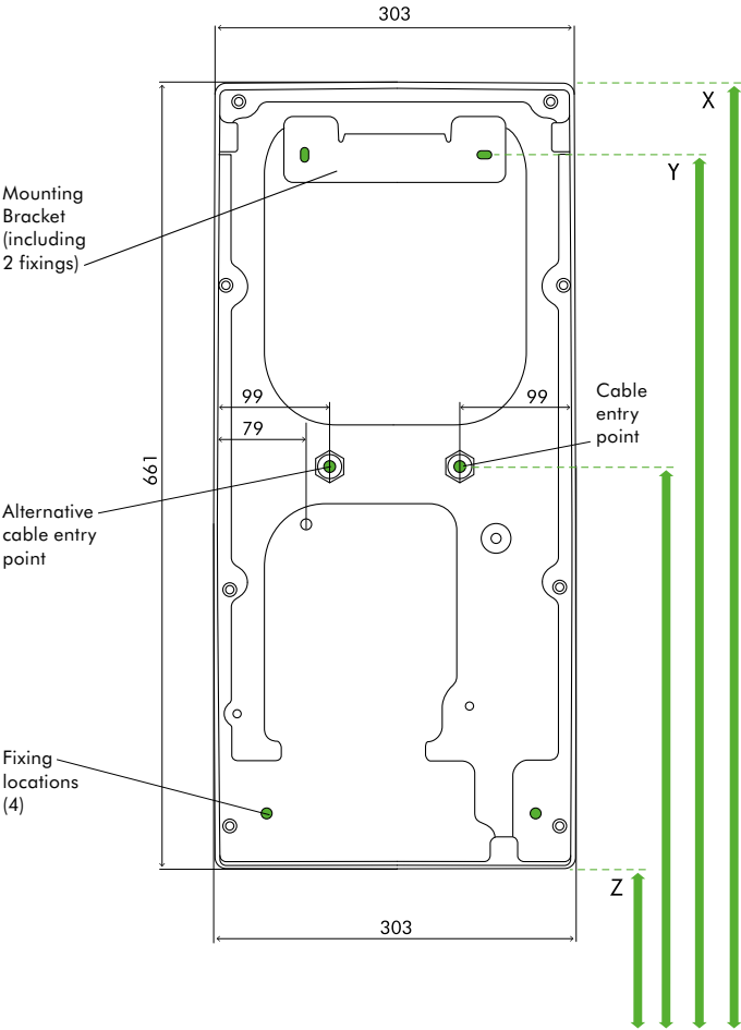
REAR ELEVATION
