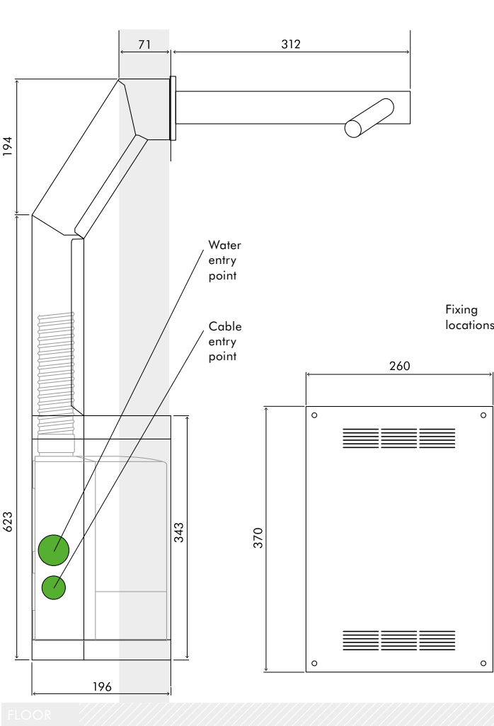
SIDE ELEVATION
