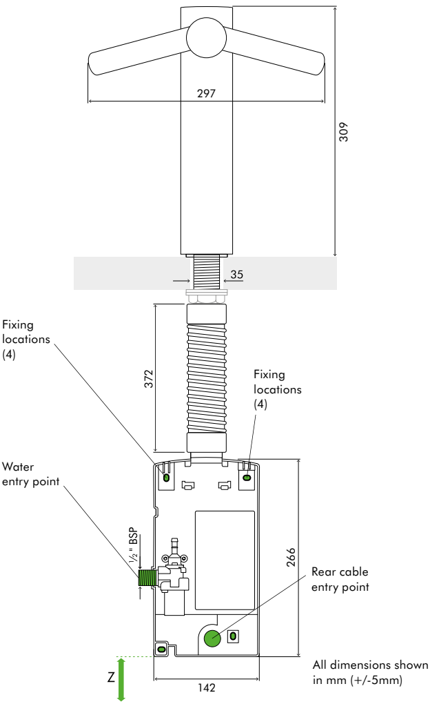
REAR ELEVATION
