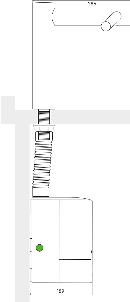
SIDE ELEVATION
