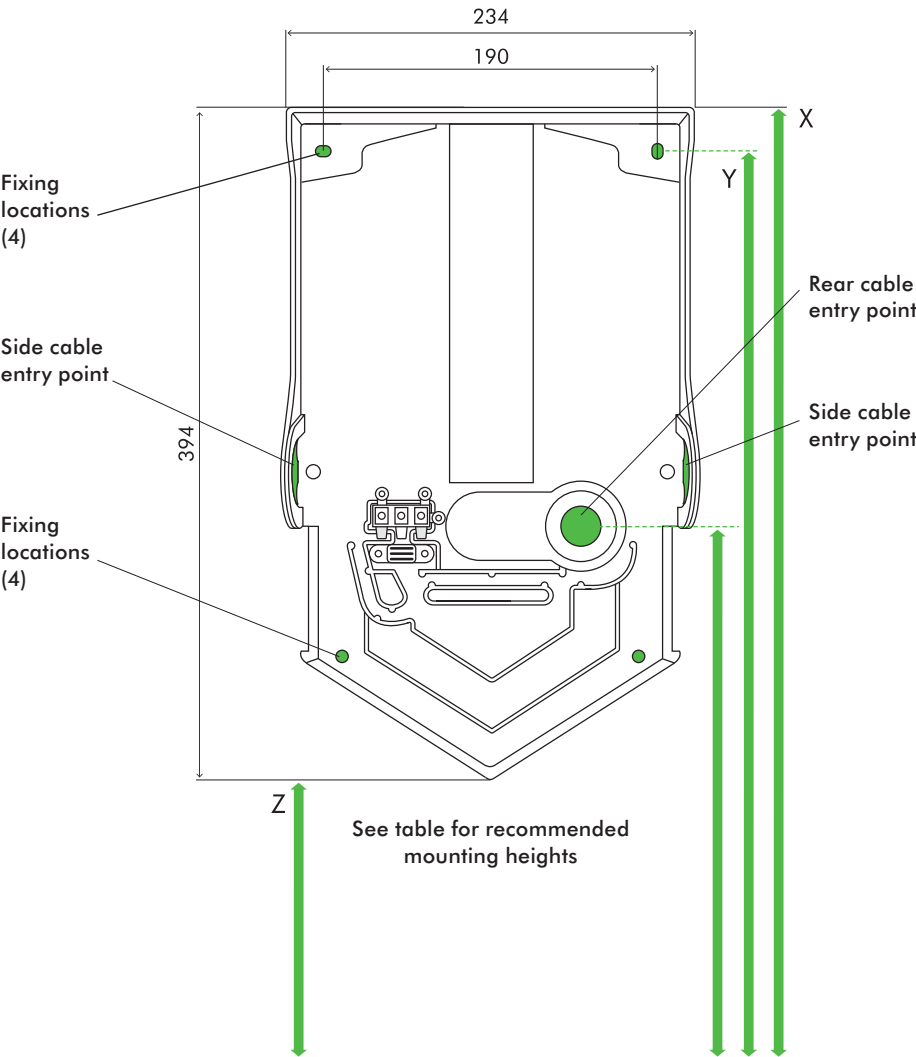
REAR ELEVATION
