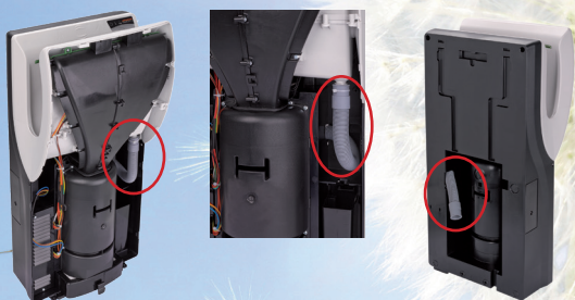
KITDESM14A Optional kit for a direct connection to the waste pipe
