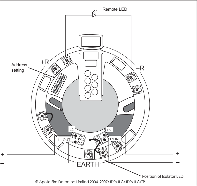
Fig. 1 Discovery Sounder Base with isolator wiring
