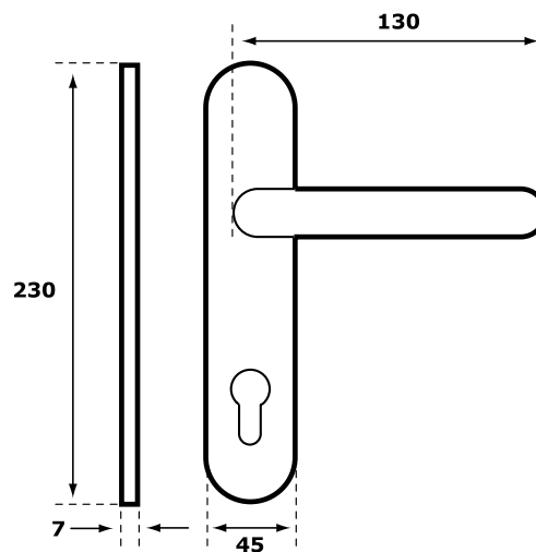
Lever on longplate
