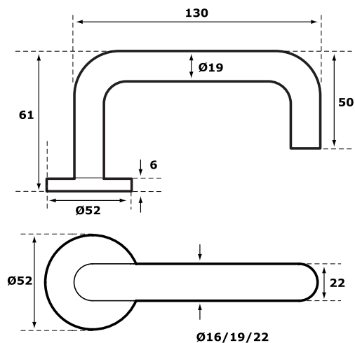
Lever on round nose
