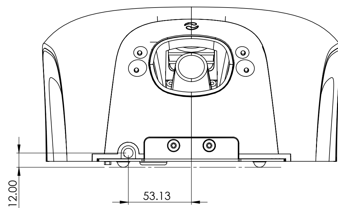
LOWER CABLE ENTRY POINT (SURFACE TRUNKING)
