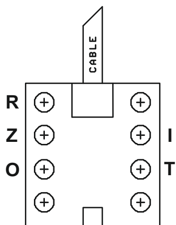
Surface box (viewed from the screws side)
