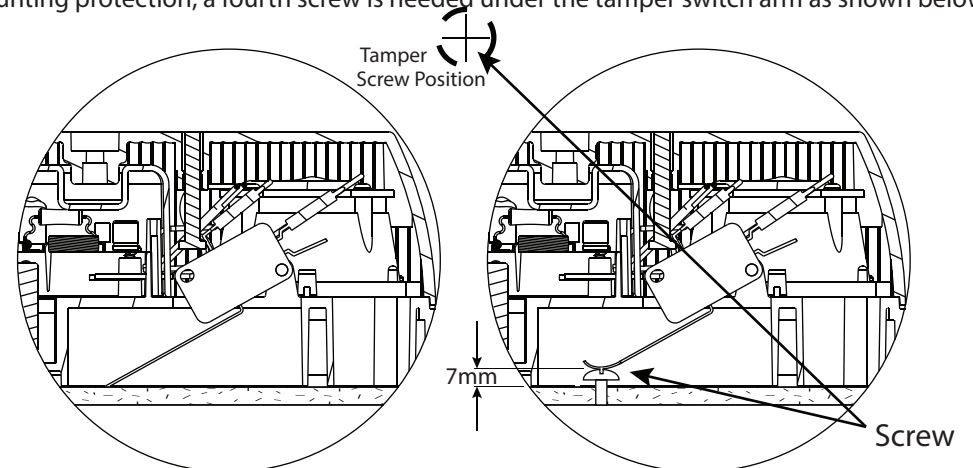
Normal Installation
