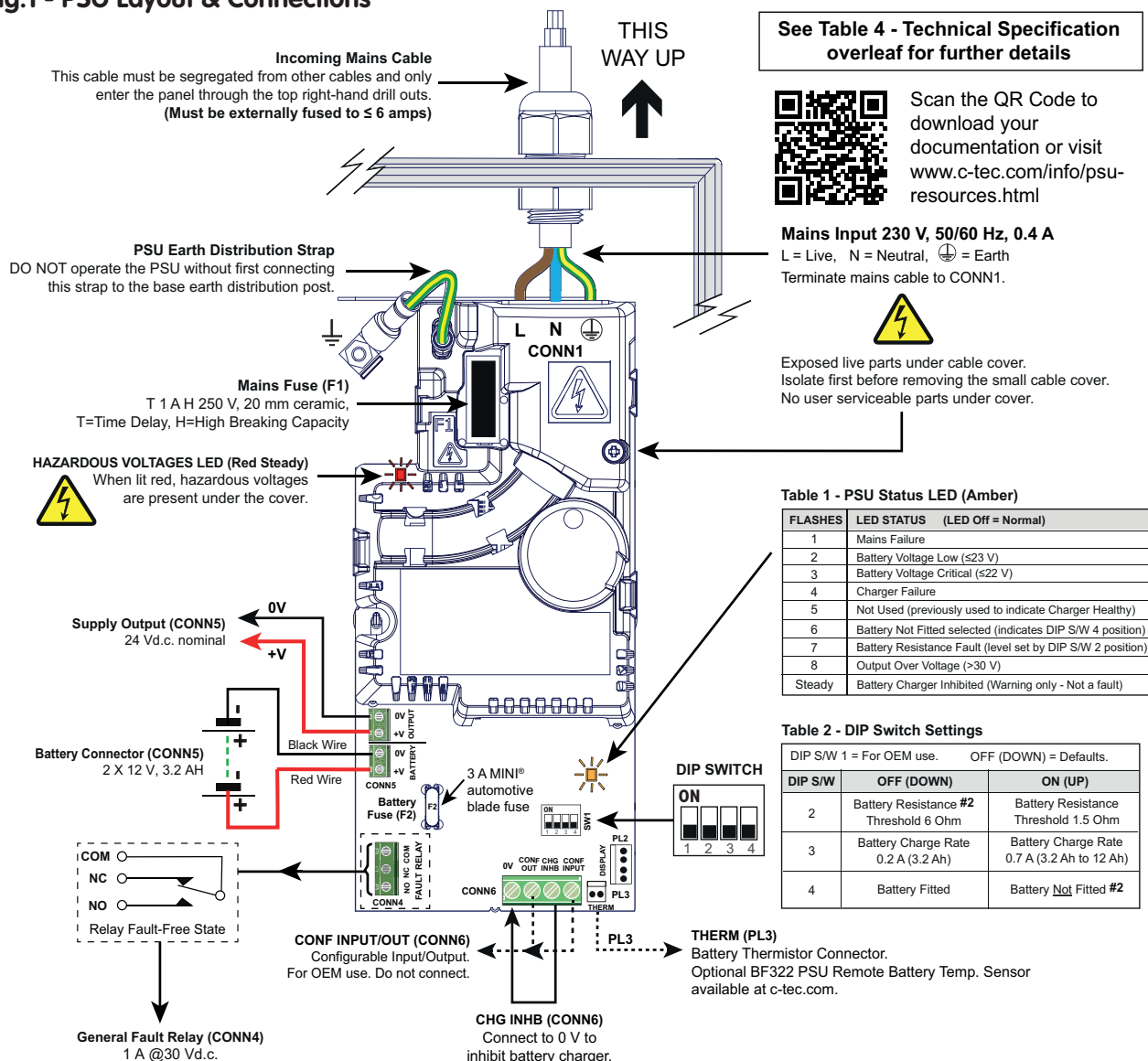
Fig.1 - PSU Layout & Connections
