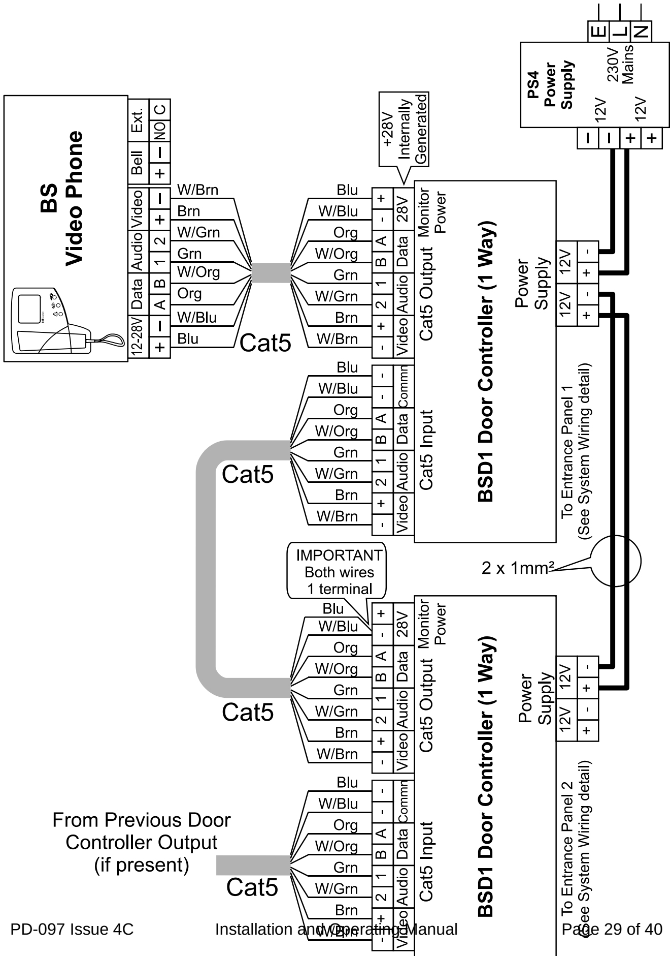
Diagram D – 1 Way Multiple Entrance Wiring Detail
