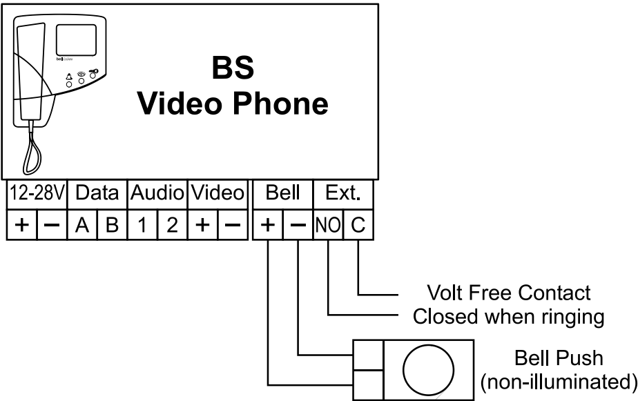
Diagram H – Videophone Connections
