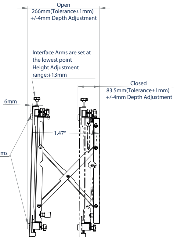
SIDE VIEW EXTENDED
