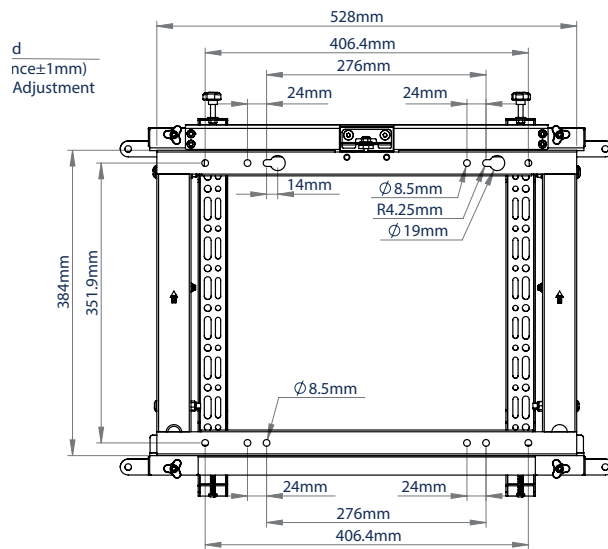
REAR VIEW
