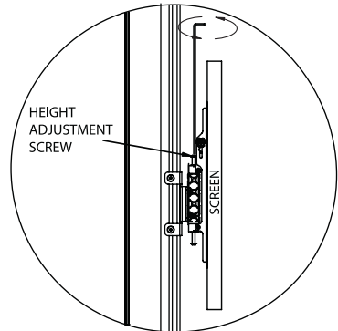
C & D MICRO-ADJUSTMENT ARMS
