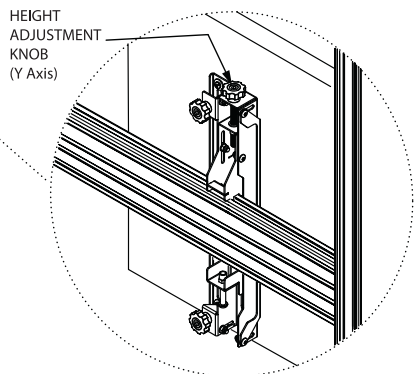
C & D MICRO-ADJUSTMENT ARMS
