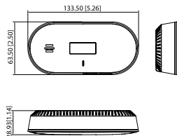
Figure 3-3 Dimensions (mm)
