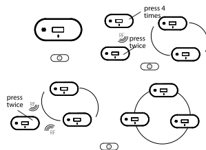
Figure 5-1 Interconnect device
