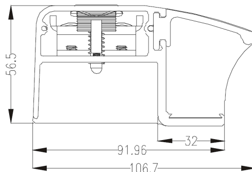
Handle Profile
