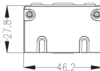
Magnet Profile
