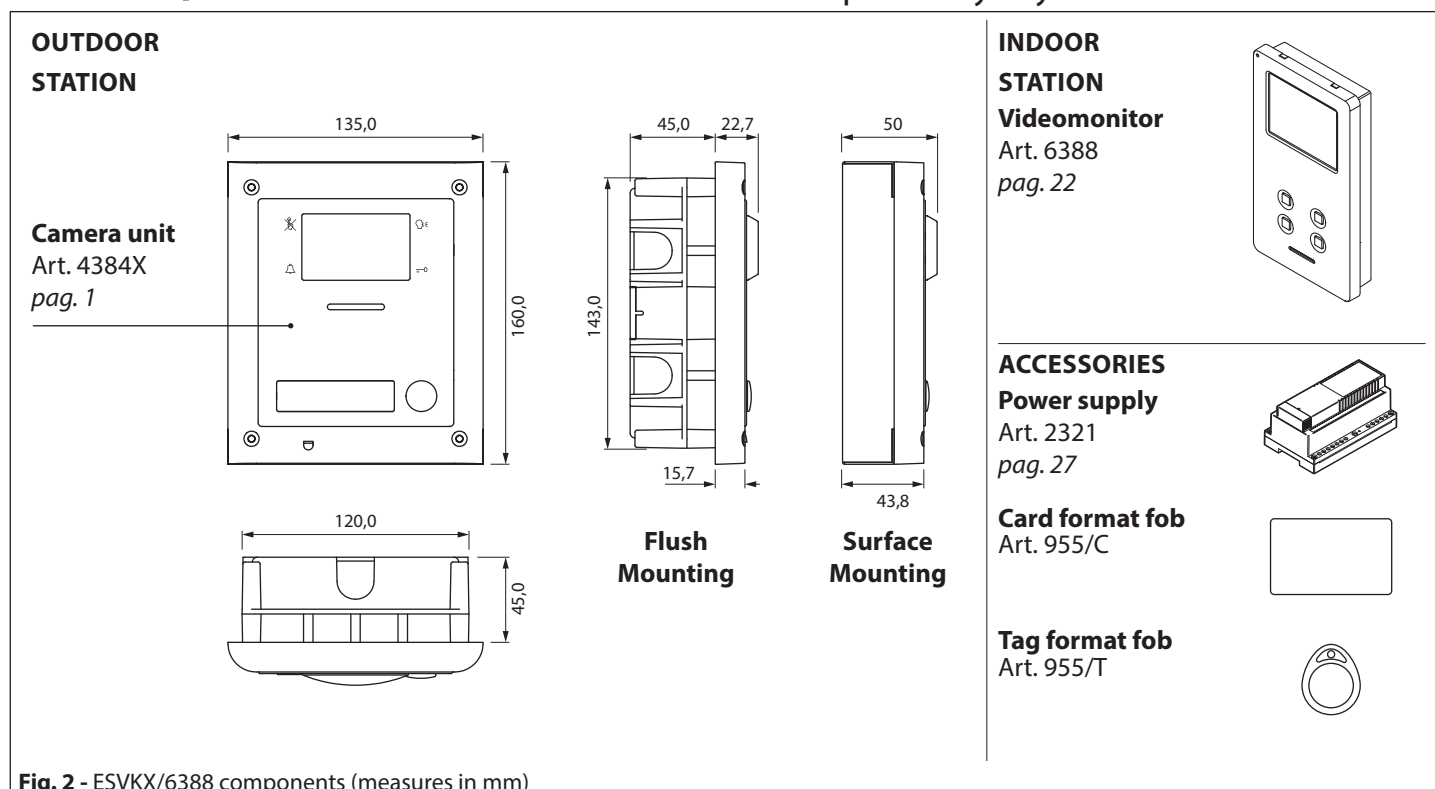
Fig. 2 - ESVKX/6388 components (measures in mm)
