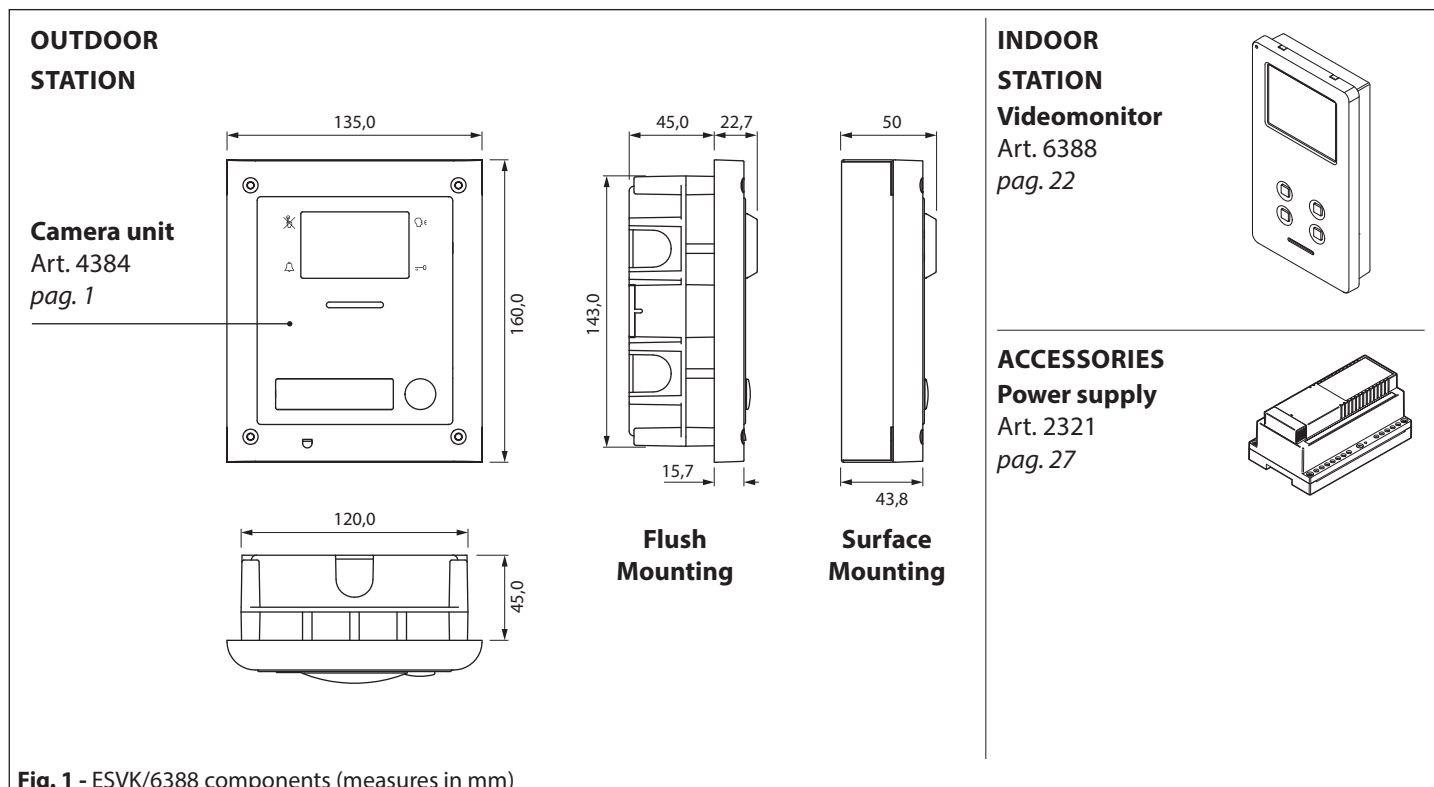
Fig. 1 - ESVK/6388 components (measures in mm)
