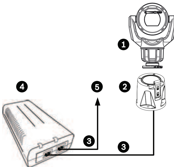
Figure 14.1: System Configuration with a midspan (no input or output connections)
