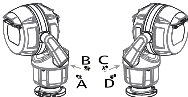
Figure 12.5: Reinsert the screws in the yoke arms in the following sequence: ABCD.
