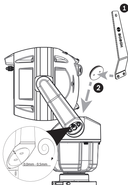
Figure 12.6: Attach the yoke caps.
