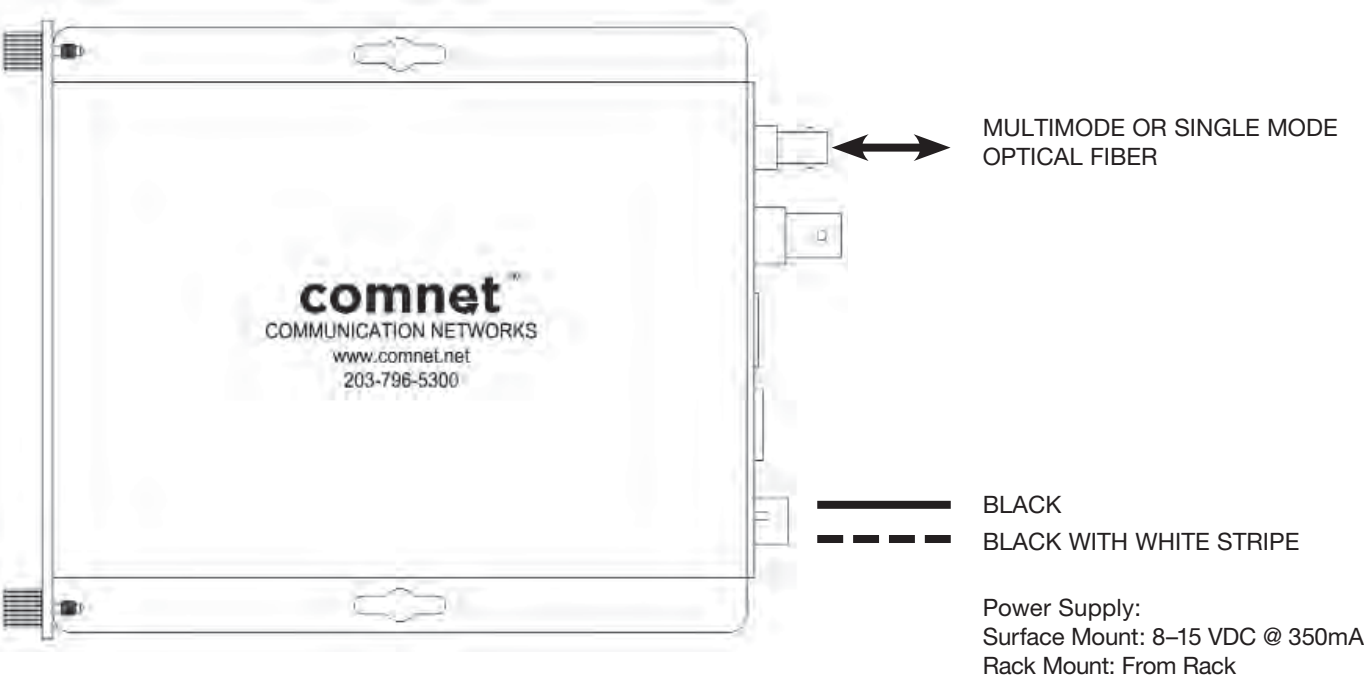
FIGURE 1 – FVT/FVR10D1E TRANSMITTER AND RECEIVER
