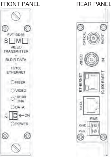
FIGURE 2 – FVT10D1E TRANSMITTER
