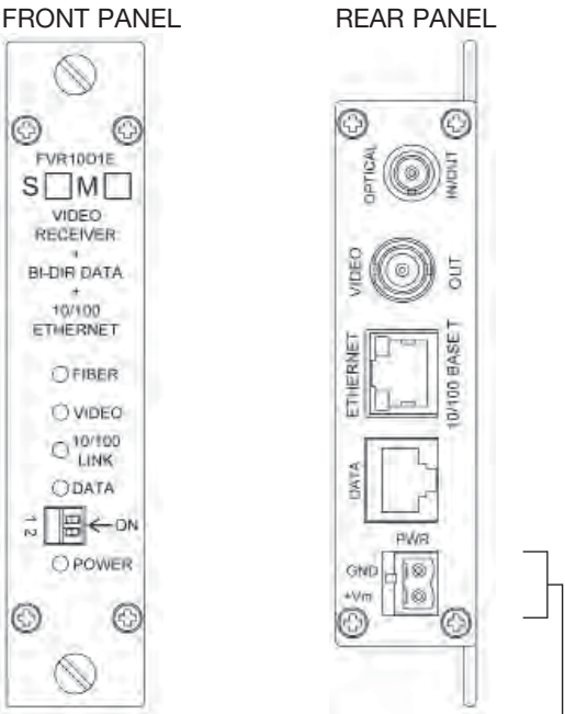
FIGURE 3 – FVR10D1E RECEIVER
