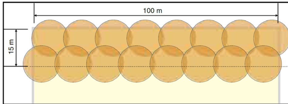
Point detector coverage over beam detector maximum area.
