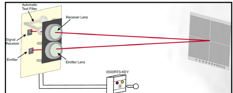
Notifier Opal Beam Detector remote test operation
