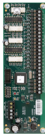
16 Channel Input/Output Board (K560)
