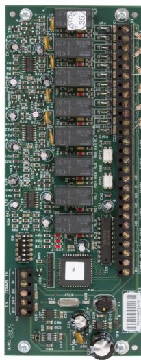
6 Way Sounder Extender Board (K546)
