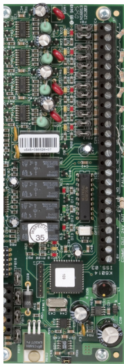
4 Way Conventional Detection Zone Module (K545)
