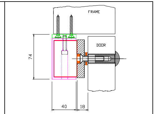
Outward opening with large reveal
