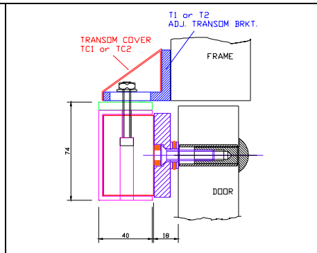
Outward opening with no reveal using adjustable transom bracket T1/T2 with cover TC1/TC2
