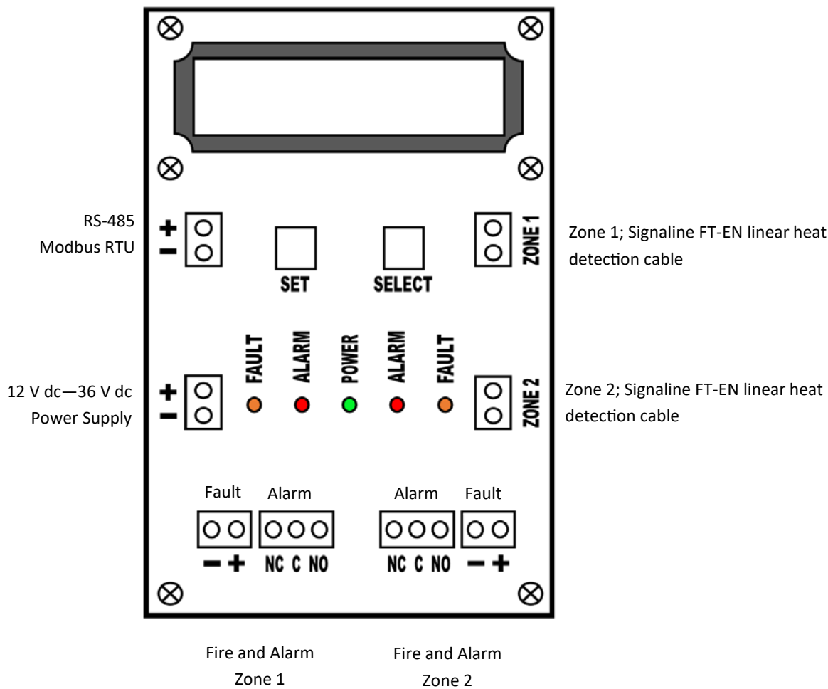
Fig. 2. Connection diagram for the Signaline LocatorPlus-EN
