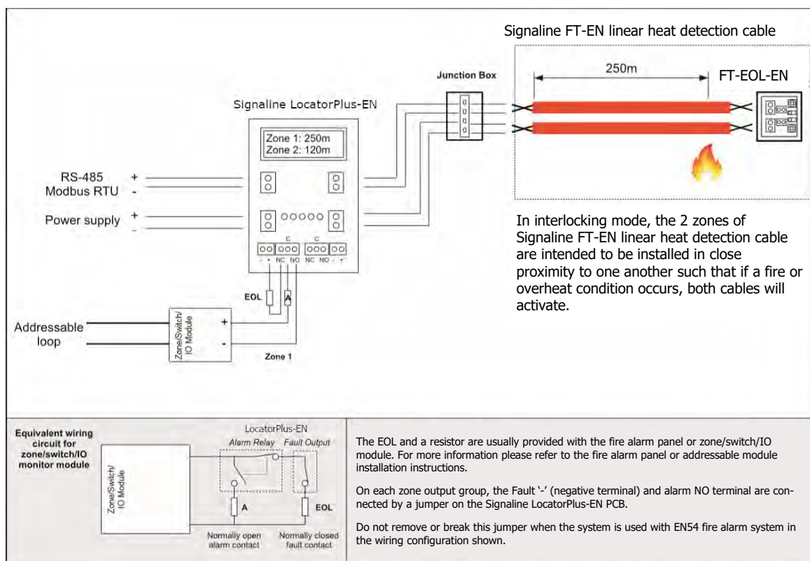
Fig. 4. Typical Schematic for interlocking operating mode
