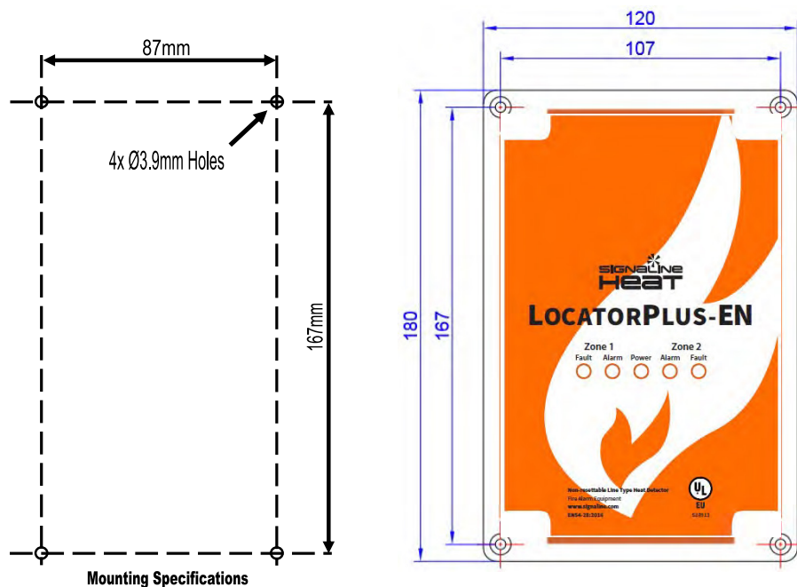
Fig. 5. Mounting specification for Signaline LocatorPlus-EN
