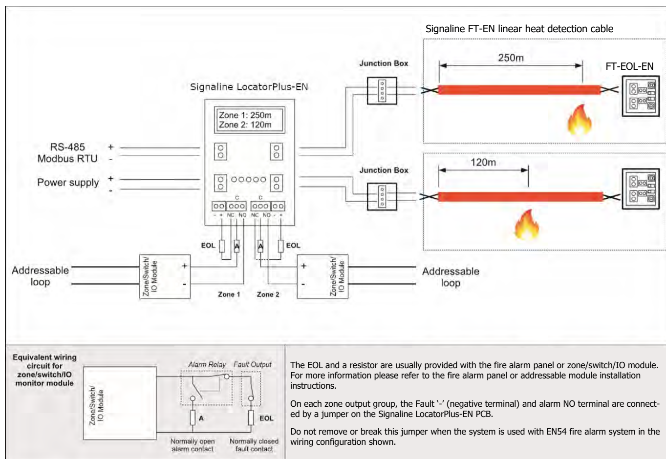
Fig. 3. Typical Schematic for independent operating mode
