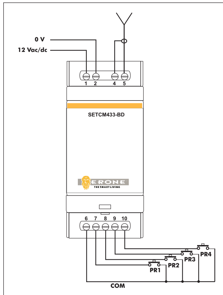
Connection diagram
